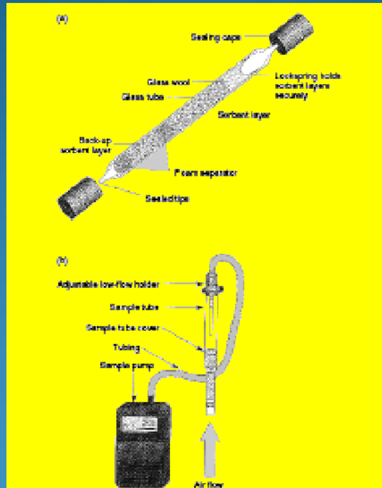
Figure 3.5 Air sampling: (a) a typical sorbent tube; (b) the system used to carry out measurements [2]. From Jones, A., Duck, R., Reed, R. and Weyers, J., Practical Skills in Environmental Analysis , Prentice Hall, Harlow, UK, 2000. © Pearson Education Limited 2000, reprinted by permission of Pearson Education Limited.
