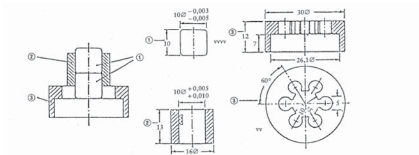
Fig. 4c Shock device for substances in powdered or paste-like form
