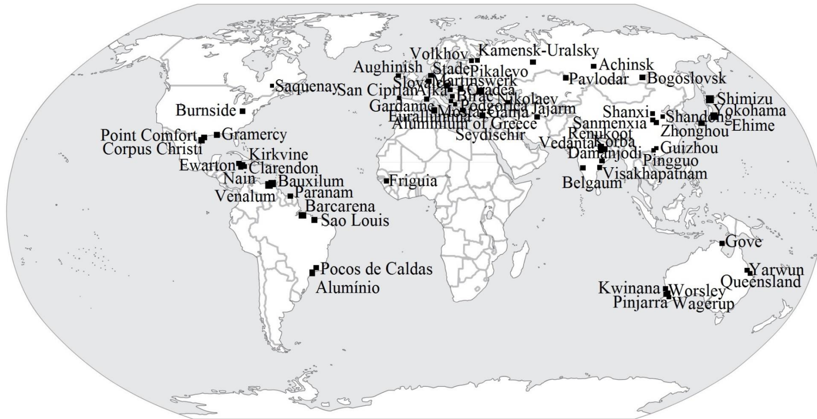
Map: World map showing the distribution of alumina refineries (Source of data: Power et al., 2011)
